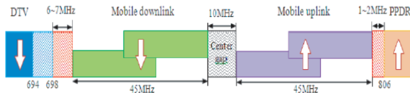
Fig. 1. FDD mode in FCA by APT.
