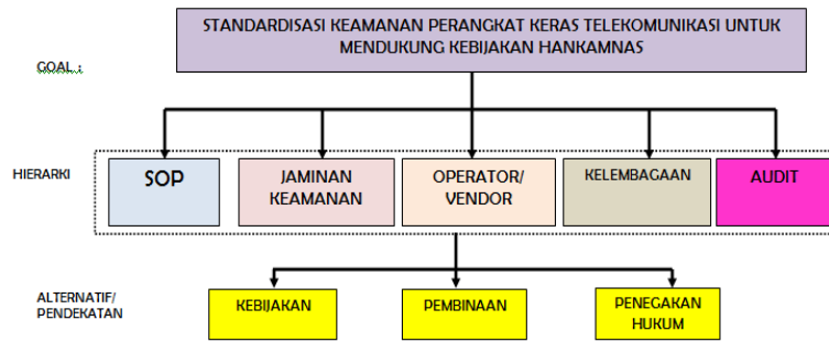
Gambar 3. Analisis AHP
