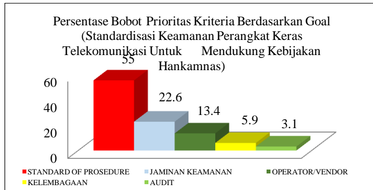
Gambar 4. Hasil AHP-Persentase bobot kriteria
